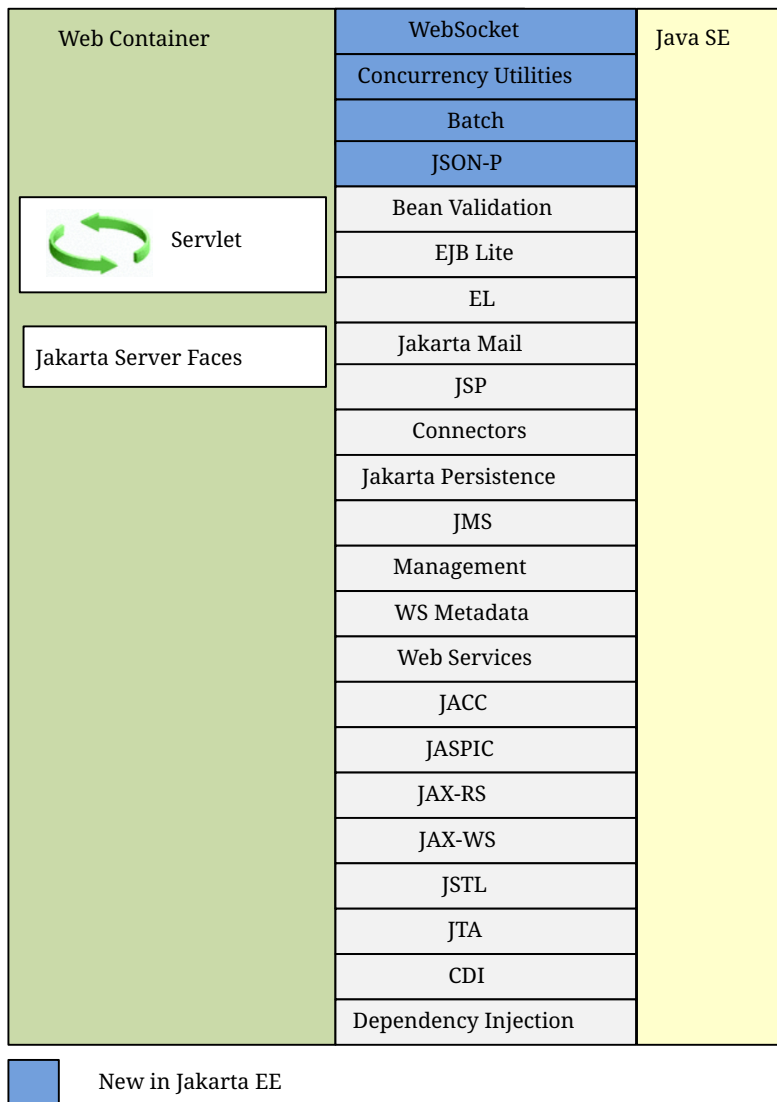
Figure 7. Jakarta EE APIs in the Web Container
