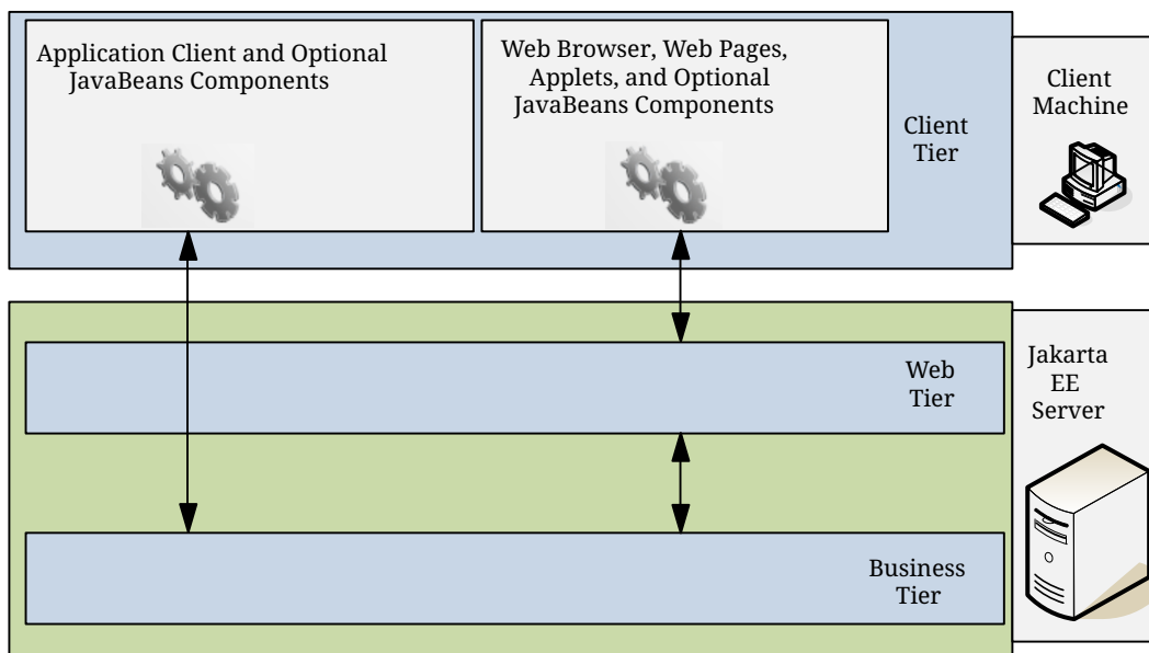
Figure 2. Server Communication
