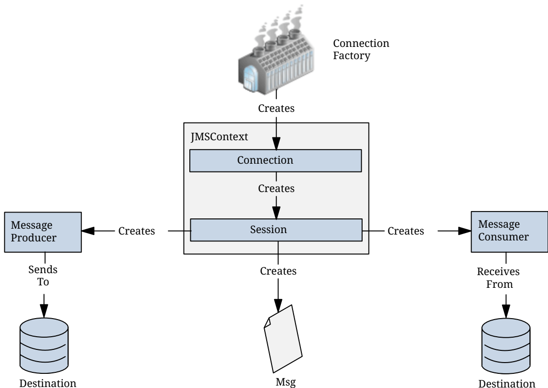
Figure 34. Jakarta Messaging Programming Model
