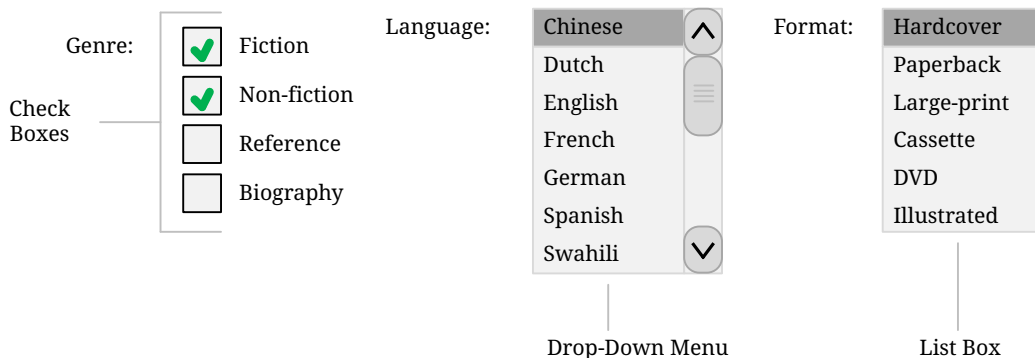
Figure 20. Example Components for Selecting Multiple Values
