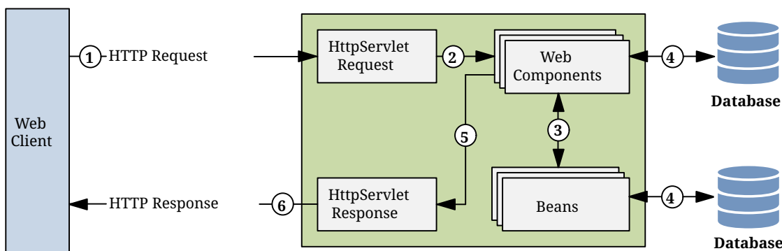
Figure 8. Jakarta Web Application Request Handling
