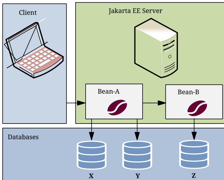
Figure 40. Updating Multiple Databases
